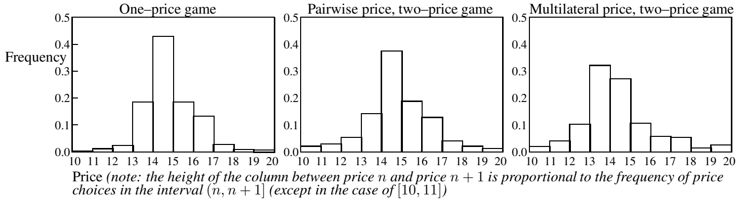
Figure 1: Histogram of prices – one-price game, two-price game (pairwise and multilateral prices)
